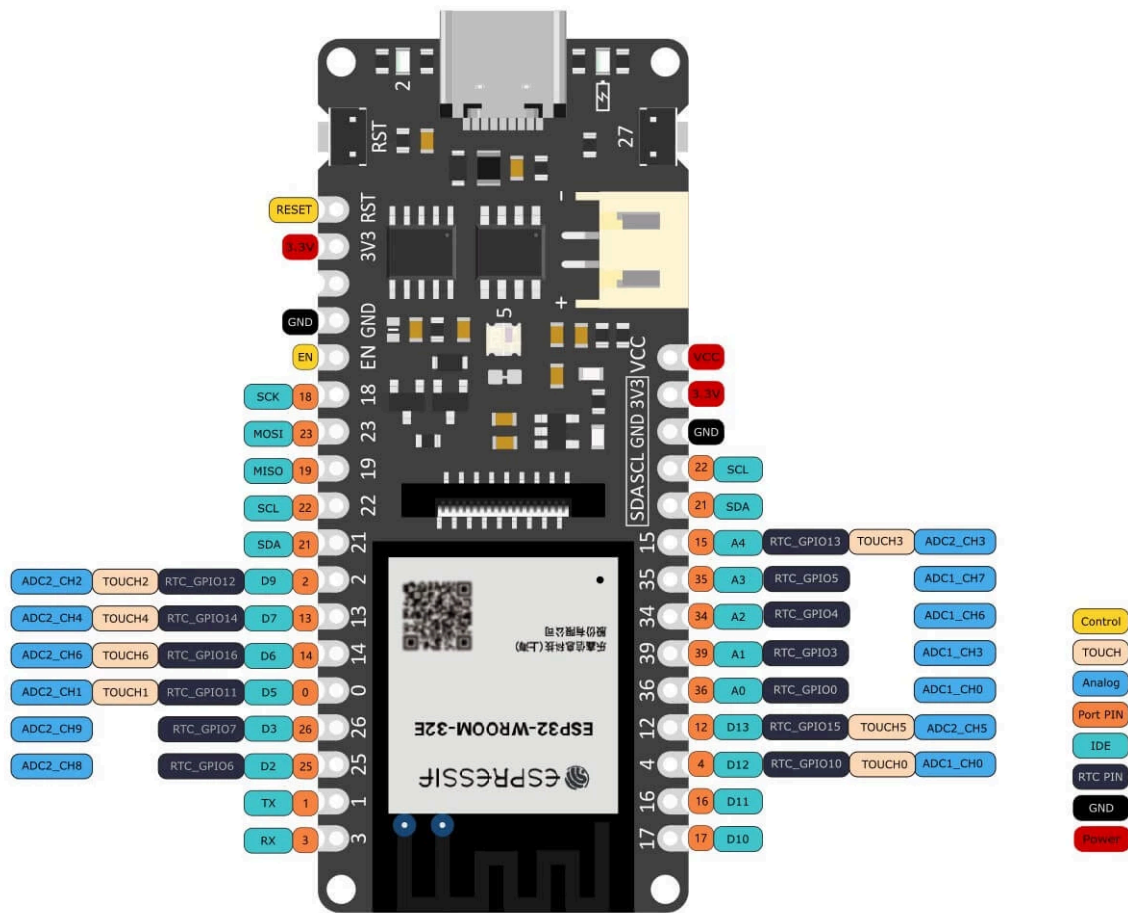
Figure 2.Pinout
