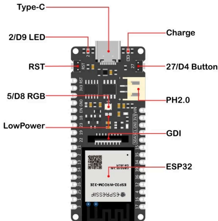
Figure 1. Board Overview
